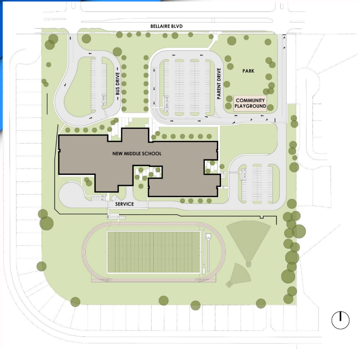
Hedrick Middle School Existing Site
