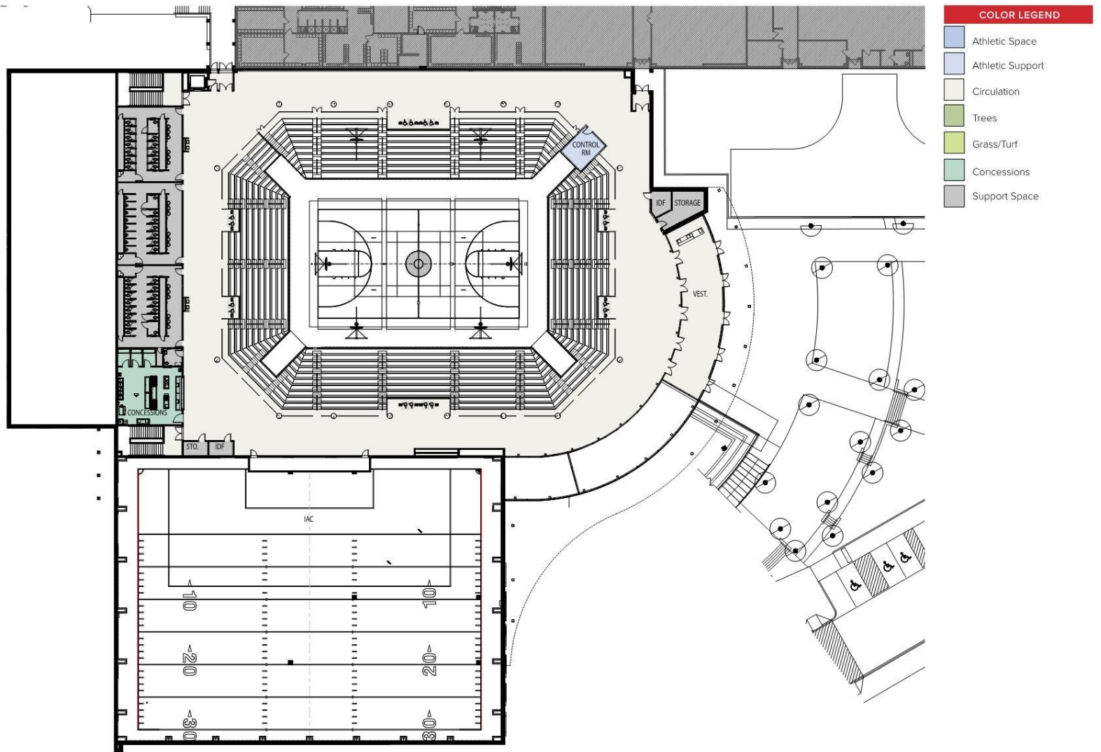
FLOORPLAN - CONCOURSE 05
